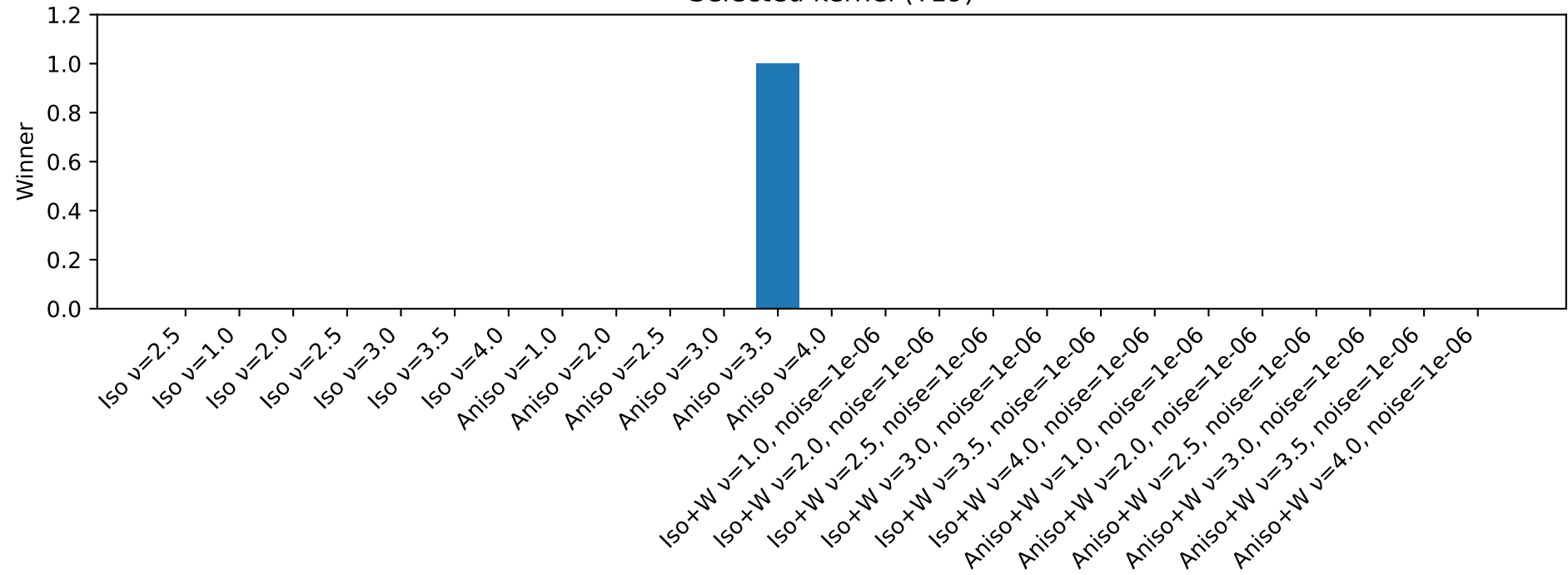
Selected kernel (T19)
