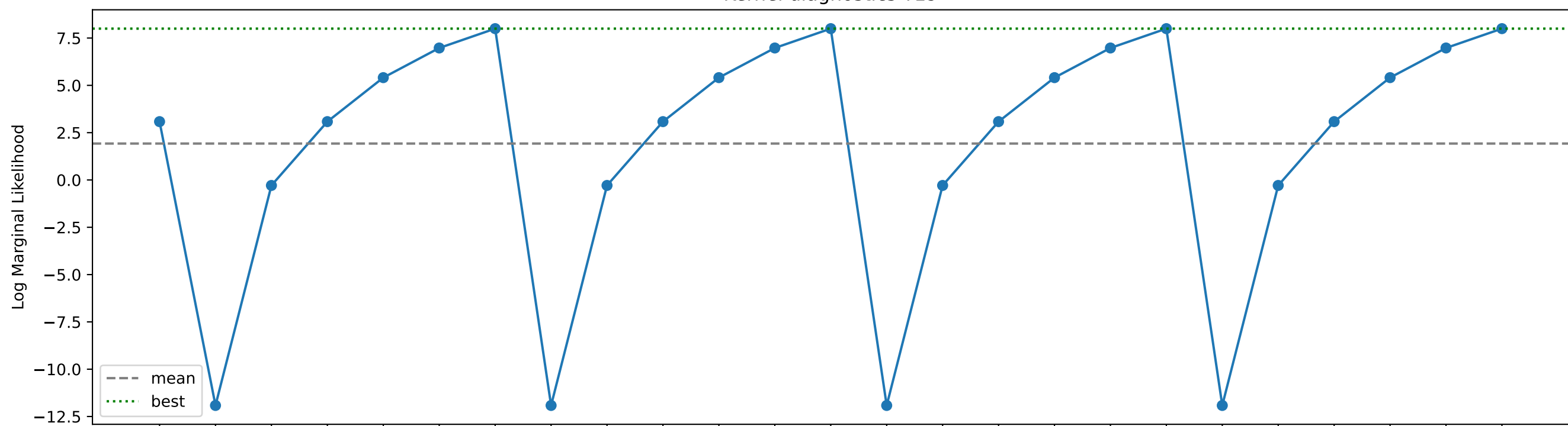
Kernel diagnostics T19
