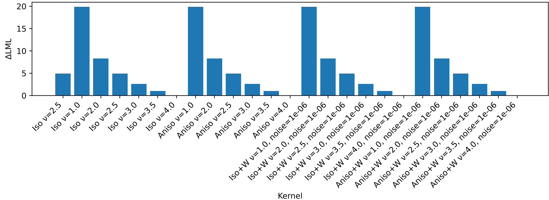
Difference from best LML (T19)
